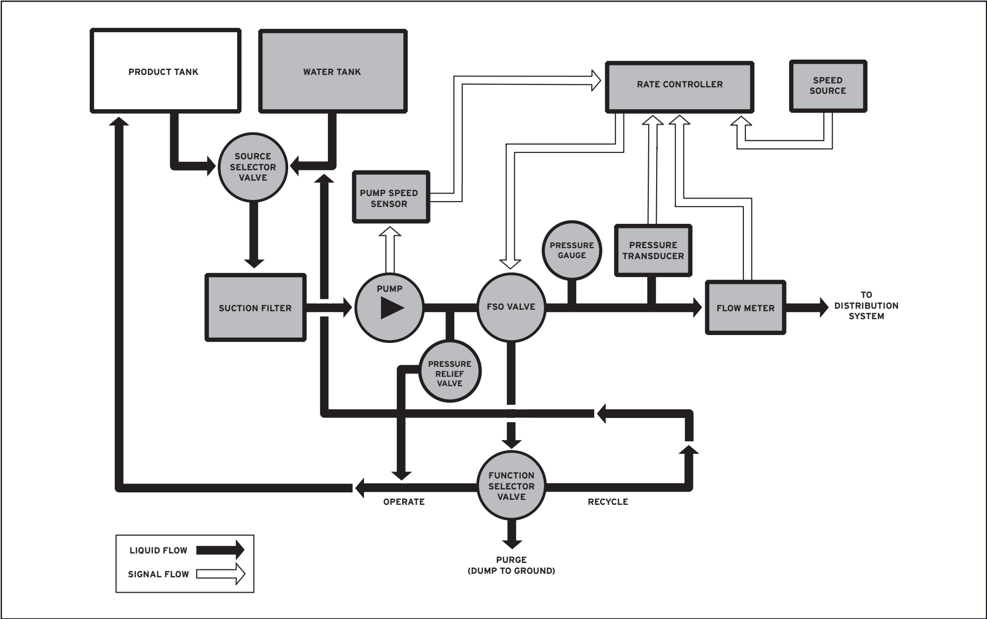
LQS70 SYSTEM LAYOUT
