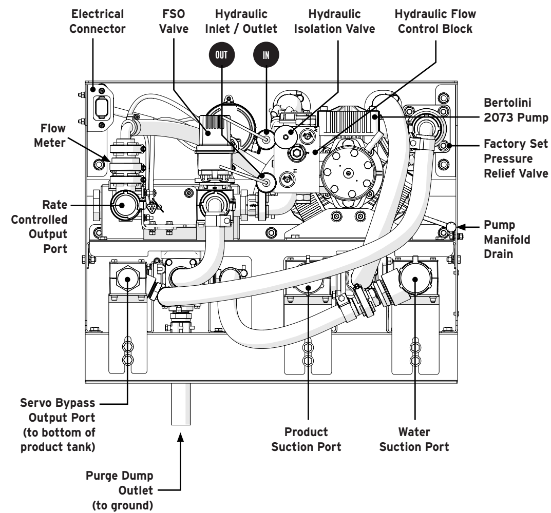
BACK VIEW
